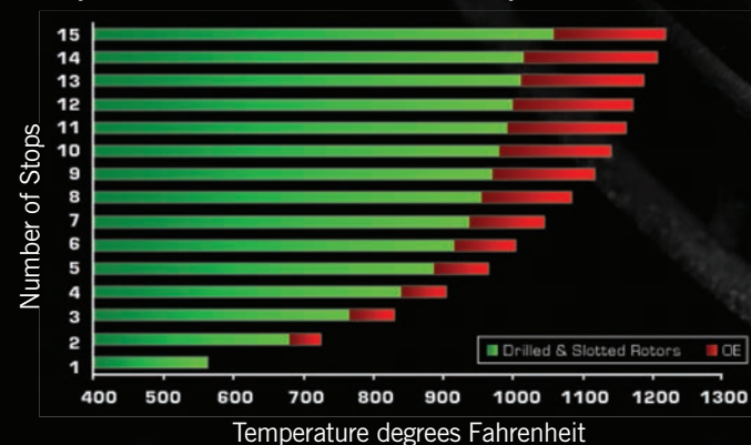
Temperature Difference Between Power Stop Drilled VS OE Rotors
